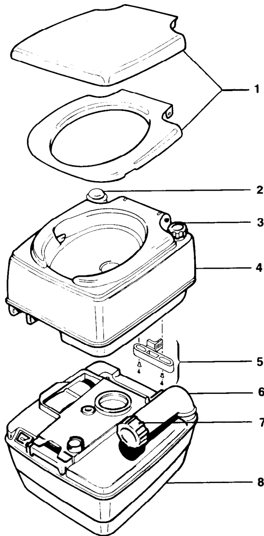
Exploded View
