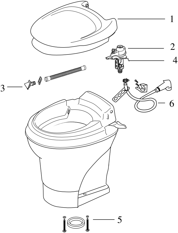
Exploded View
