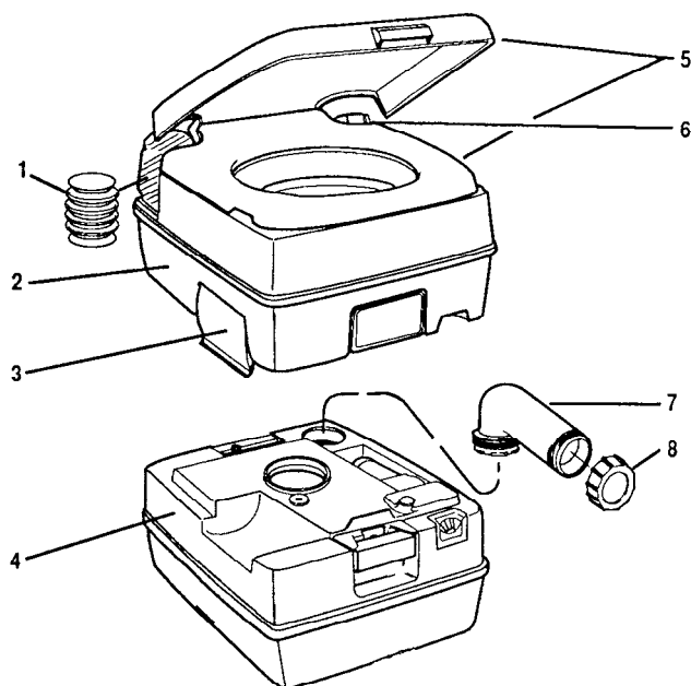
Exploded View
