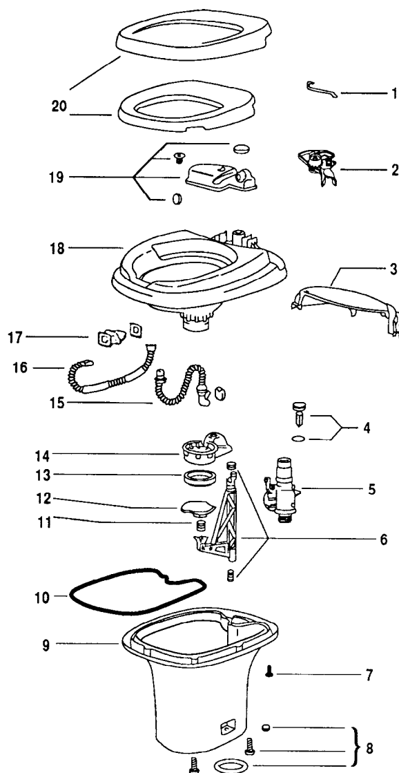
Exploded View
