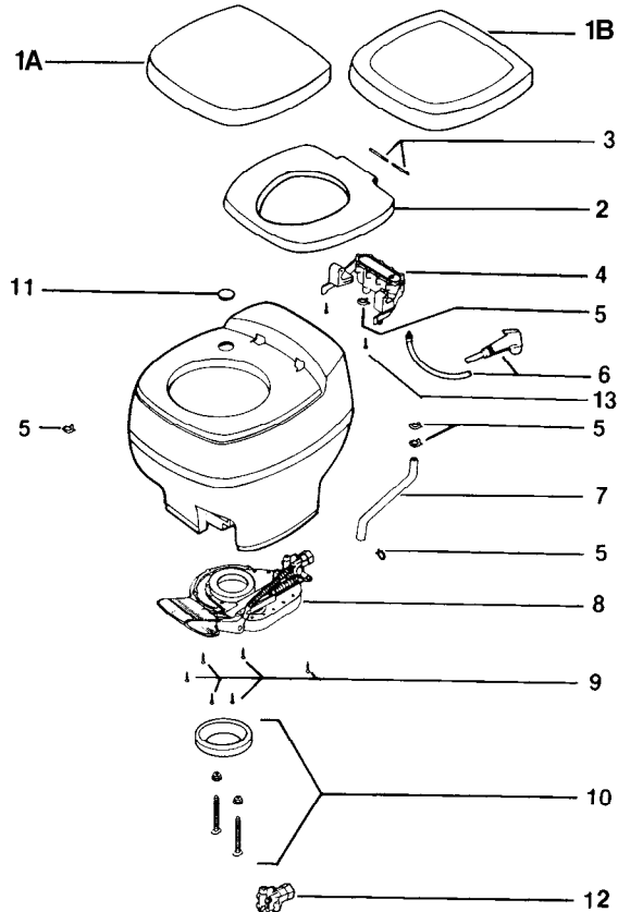
Exploded View
