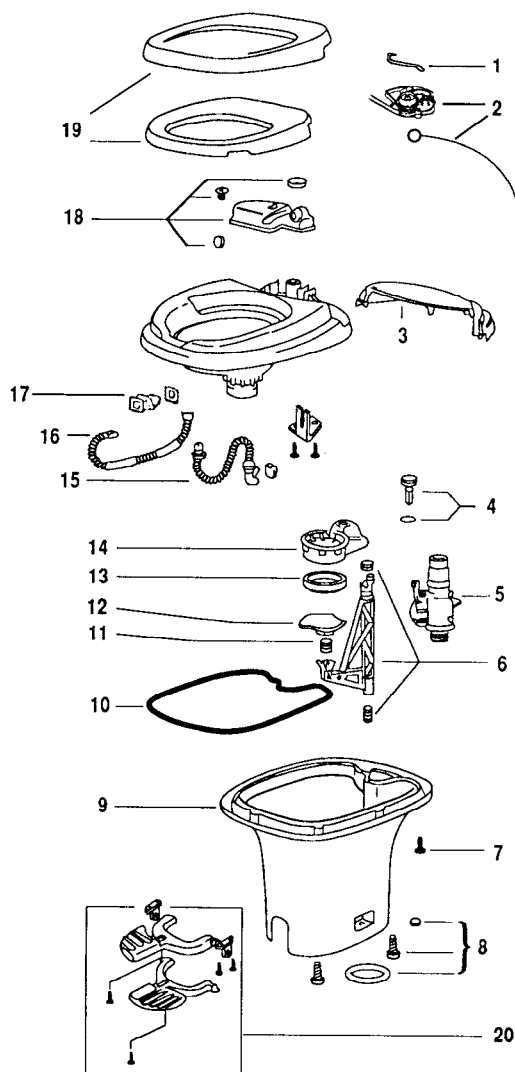
Exploded View
